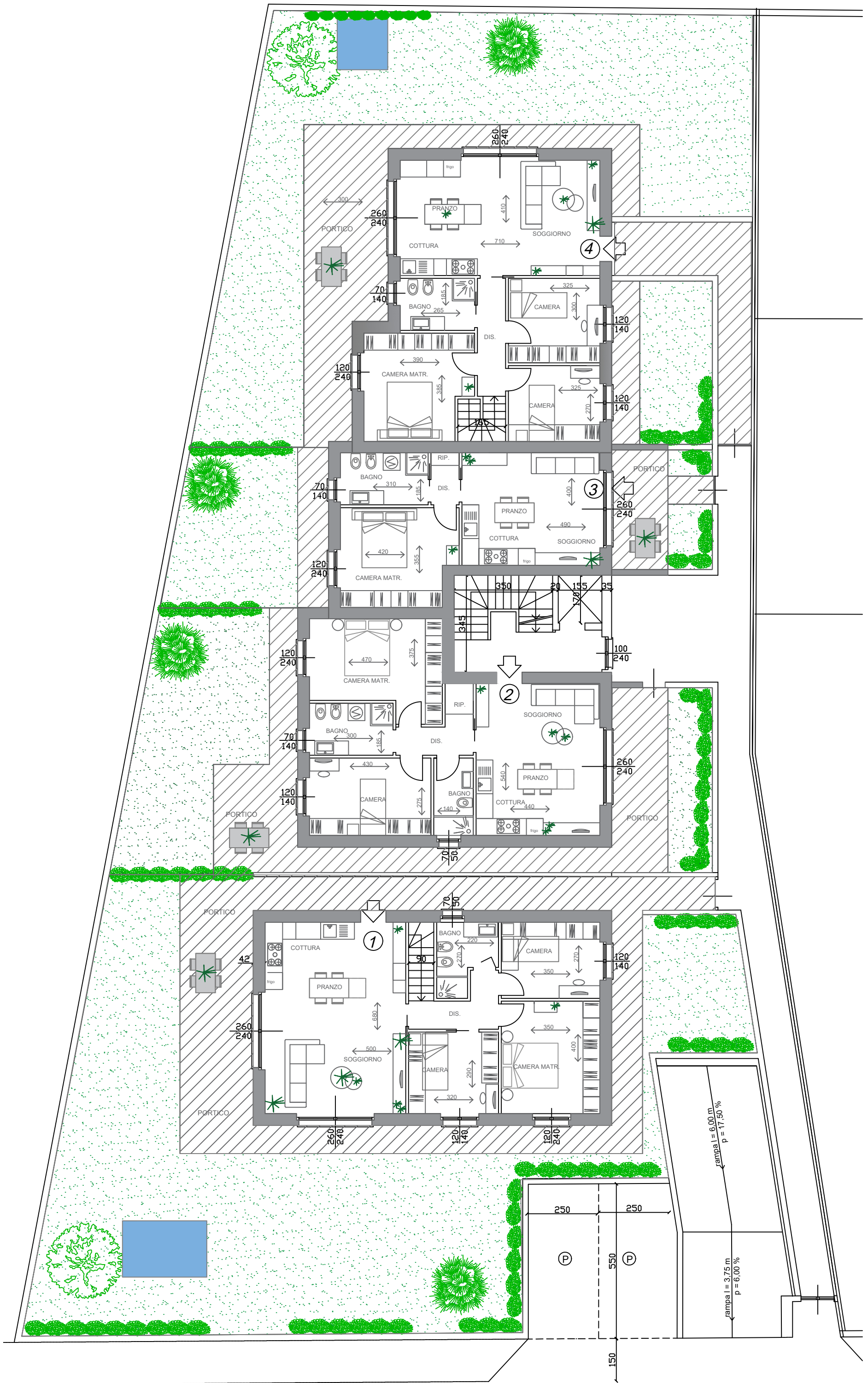
PIANO TERRA
